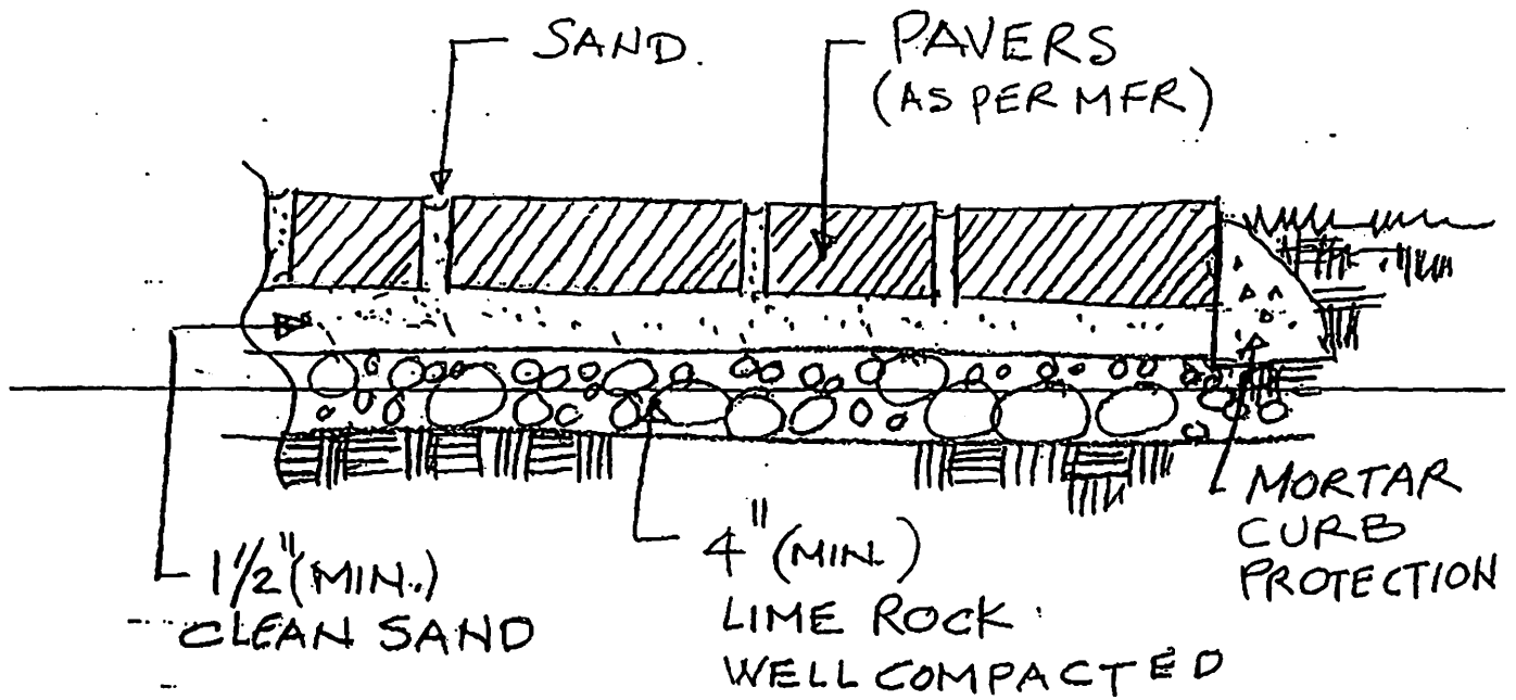
SECTION - DETAIL N.T.S. (PAVERS INSTALLATION)
