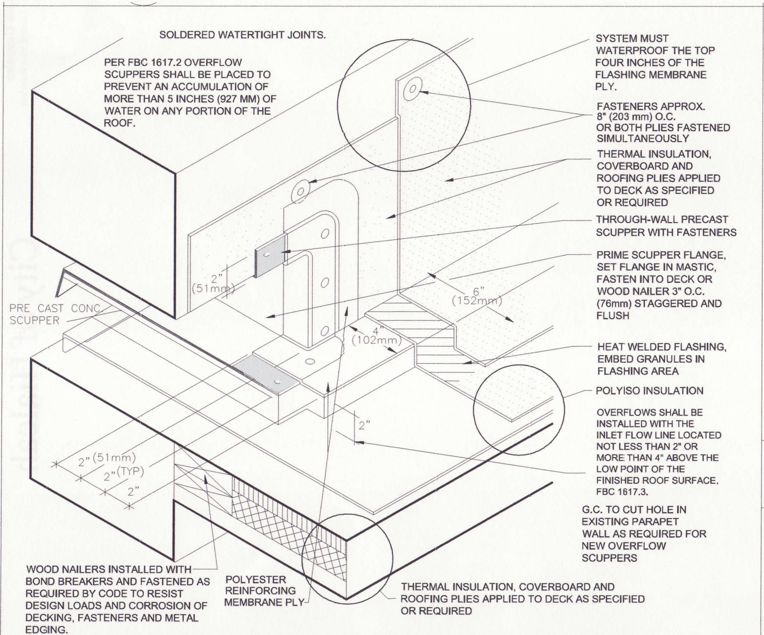
6 ROOF SCUPPER/OVERFLOW SCUPPER DETAIL AA-1.5 SCALE: 3" = 1'-0"
